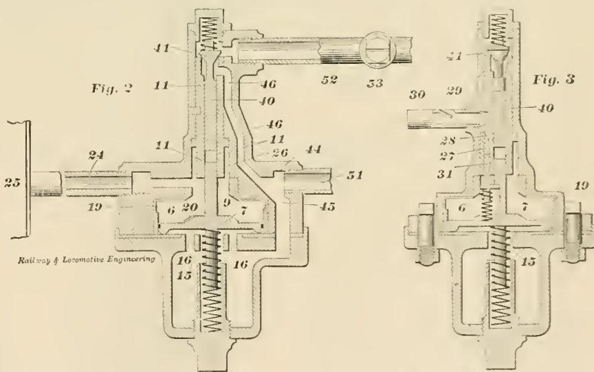
RECENTLY INVENTED AUTOMATIC DOUBLE HEADING FEED VALVE.
